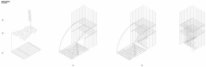
3: Mapping of the different components and assembly strategies. Studio Cabay.
